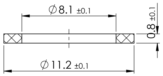
SECTION X-X
